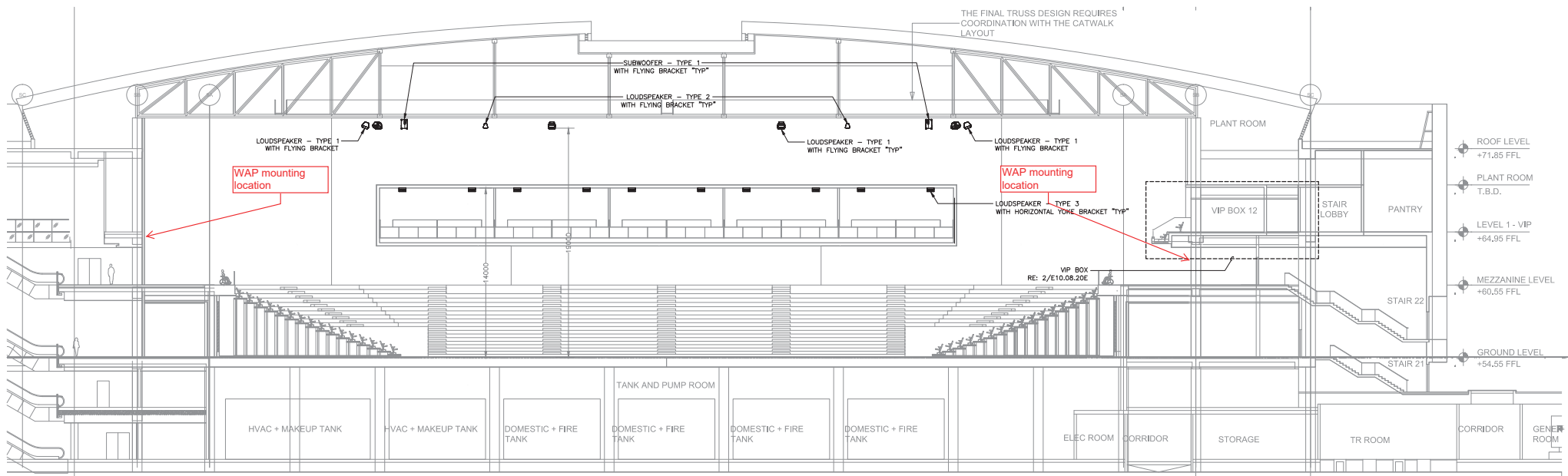
1 DETAIL - ARENA ELEVATION LAYOUT SCALE: 1/200
