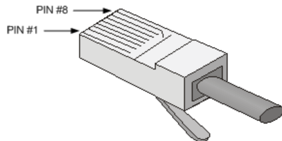
Figure 1 RJ-45 connector
